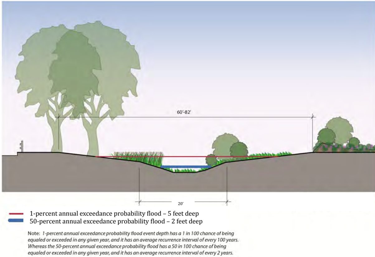
Figure 3-18. Conceptual Greenway Corridor Cross Section View with Water Depths (feet) for Different Rainfall Events
