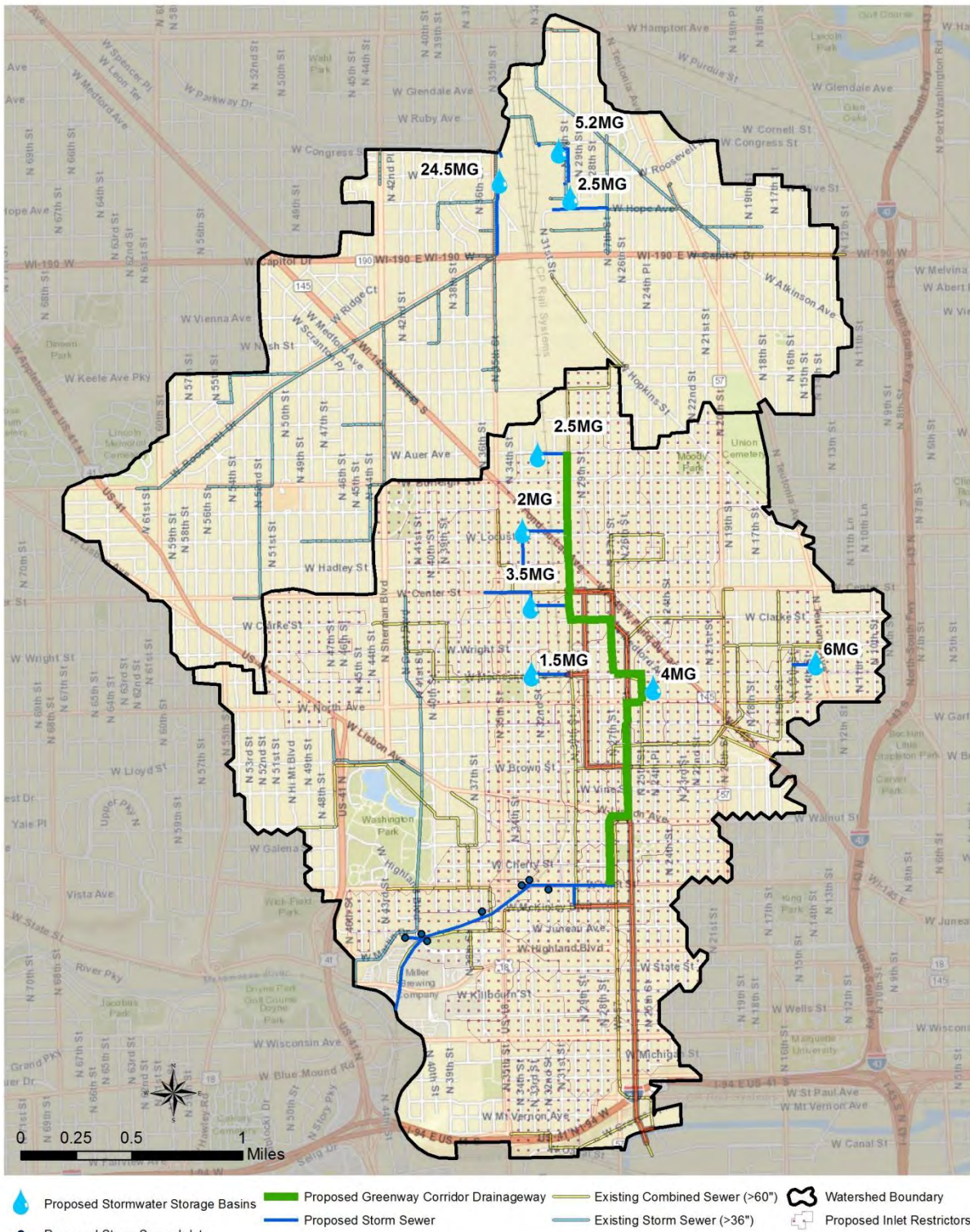
Figure 3-6. Corridor Drainage Solution Components
